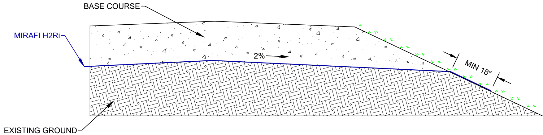
EMBANKMENT H2Ri DAYLIGHT TO VEGETATED SLOPE DETAIL NOT TO SCALE
