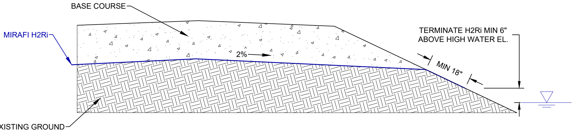
EMBANKMENT H2Ri DAYLIGHT INTO DITCH DETAIL NOT TO SCALE
