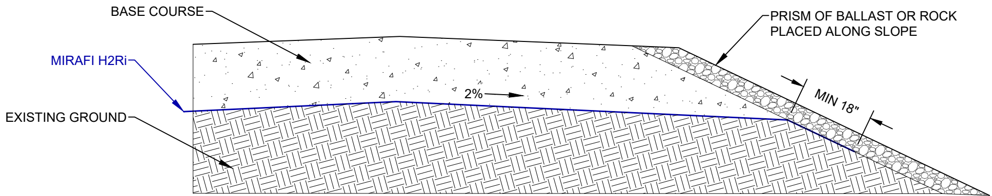
EMBANKMENT H2Ri DAYLIGHT TO BALLAST OR ROCK SLOPE DETAIL NOT TO SCALE
